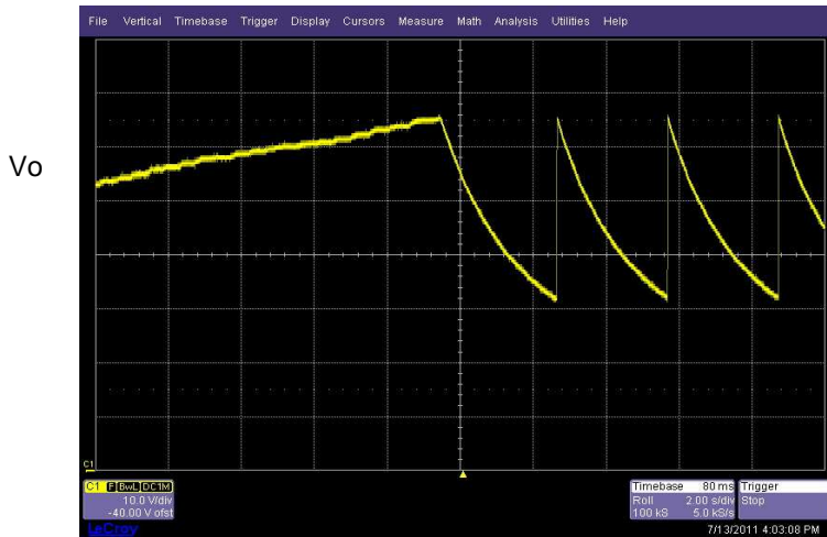
Output Voltage during OVP mode (0% Load)
