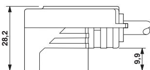
Dimensional drawing
