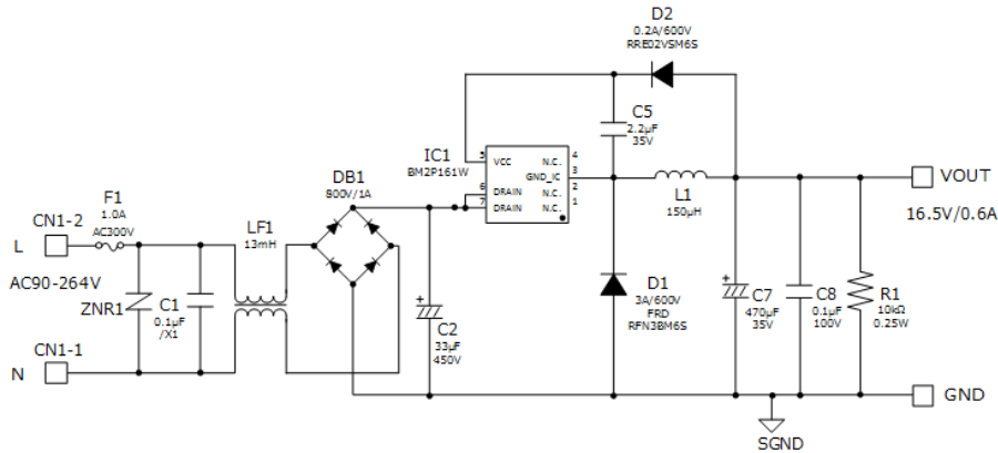
Figure 3. BM2P161W-EVK-001 Schematics
