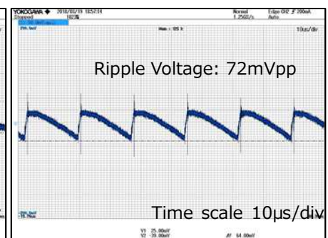
V_{IN}=230Vac , I_{OUT}=600mA
