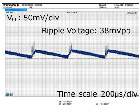
V_{IN}=230Vac , I_{OUT}=10mA
