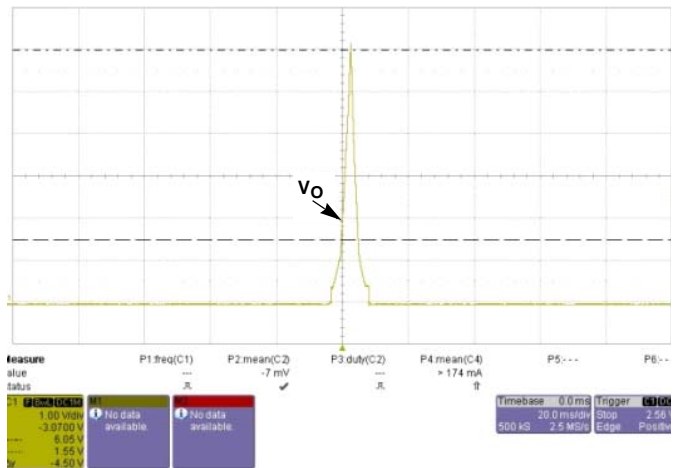
FIGURE 40. OVP @ V_{IN} = 75V, I_O = 40A
