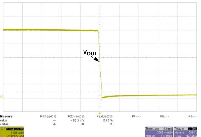
FIGURE 28. SHUT-DOWN AT V_{IN} = 75V @ I_O = 0A
