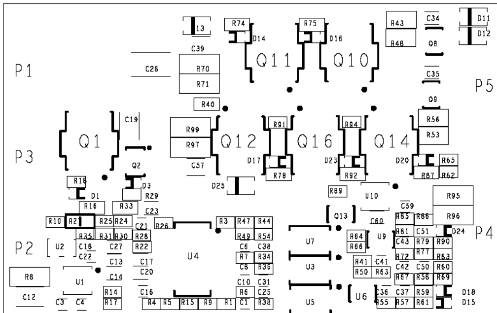
FIGURE 5. ISL6726EVAL1Z BOTTOM VIEW
