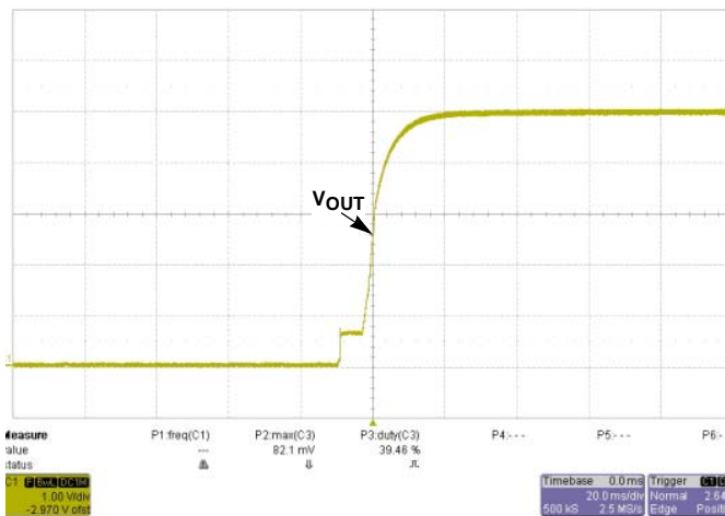
FIGURE 13. START-UP (30ms) AT V_{IN} = 48V @ I_O = 40A
