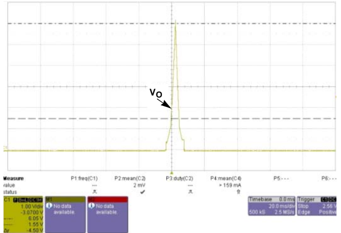
FIGURE 36. OVP @ V_{IN} = 36V, I_O = 40A
