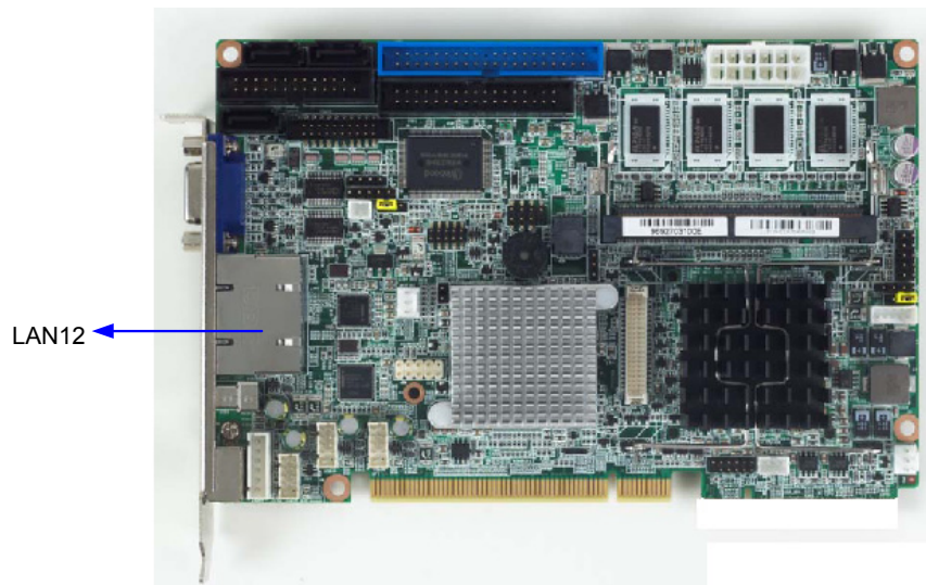
Figure 2.11 Dual Giga LAN RJ45 connector (LAN12)
