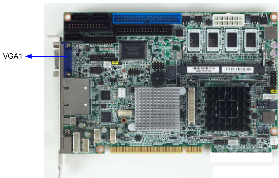
Figure 2.4 VGA Connector (VGA1)
