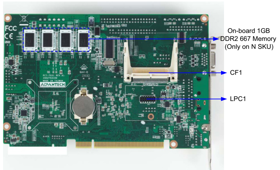
Figure 1.1 Board Layout
