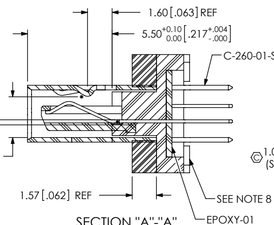
FIG 1 (MUSBS-05-S-B-TH SHOWN)
