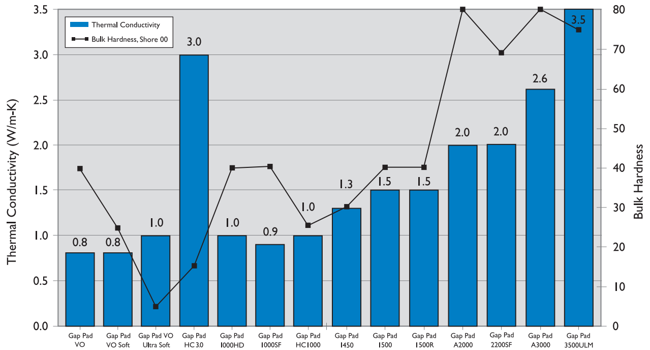
Gap Pad Thermal Conductivity vs. Hardness
